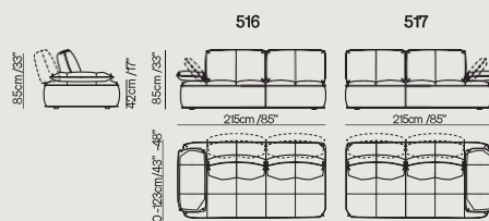
Sofa with manual adjustable backrests and arm
