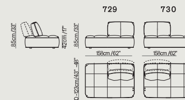
Seat with terminal and power adjustable backrest
